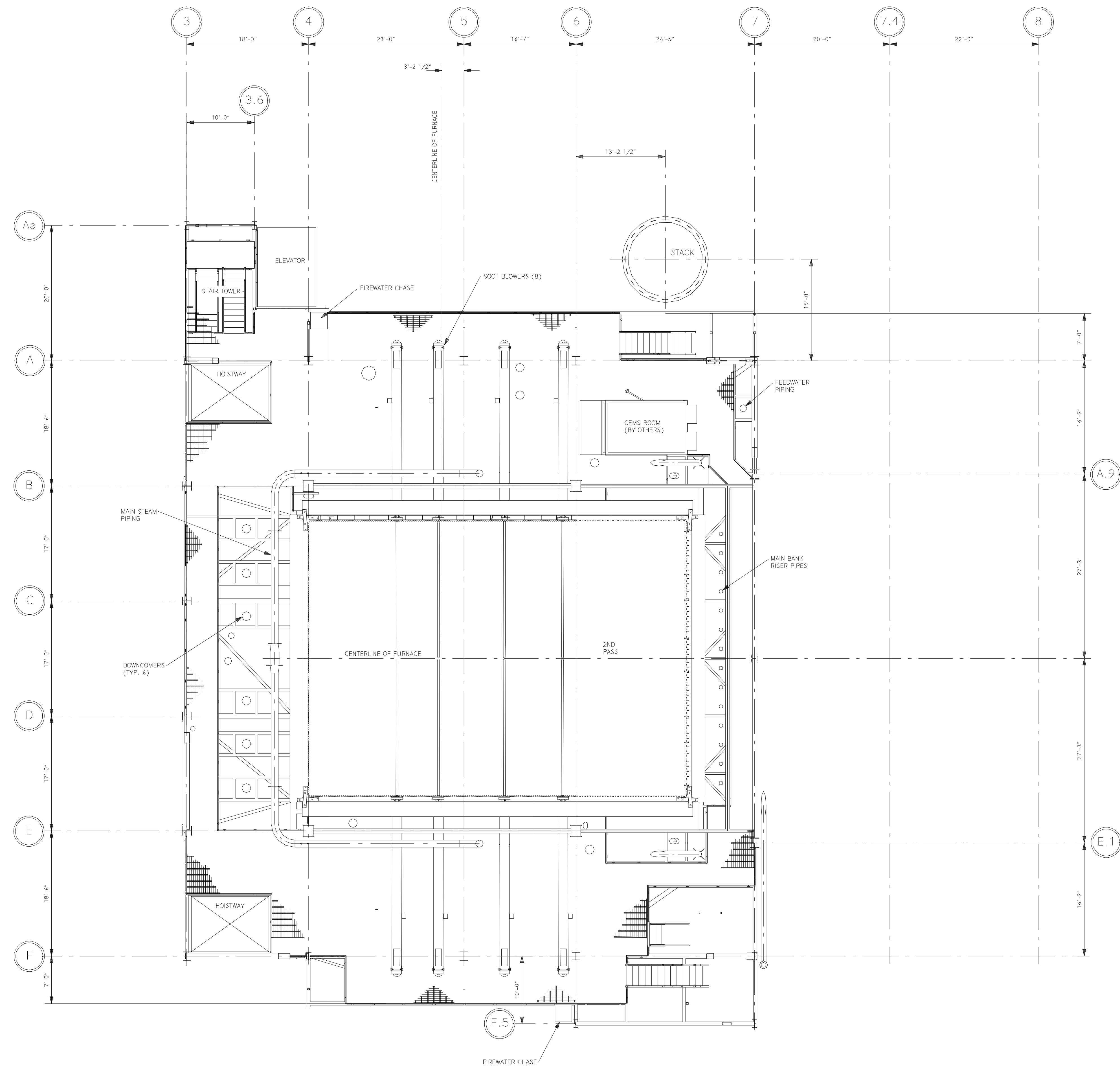
PLAN VIEW ELEVATION 333'-6"
